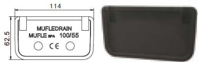
CLOSED END-CAP WITH DRAIN 100/55
