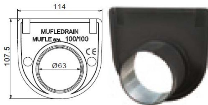
END-CAP 100/100
