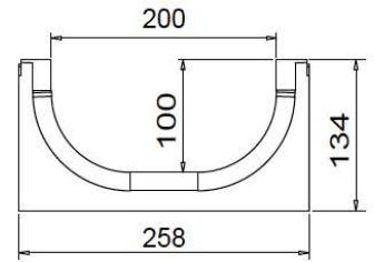
SECTION
