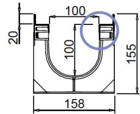
SECTION
