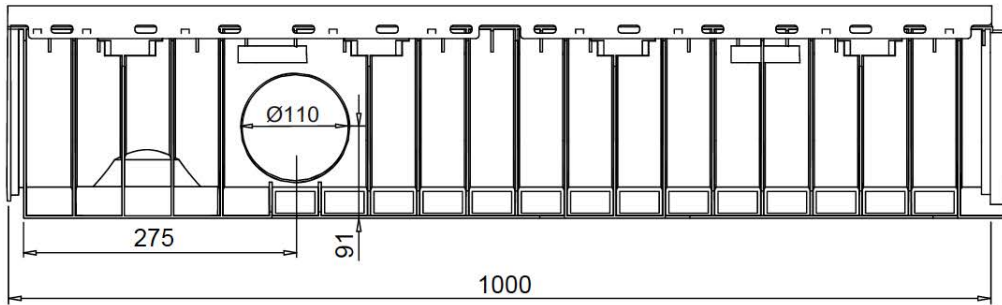
SIDE VIEW
