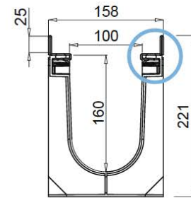
SECTION
