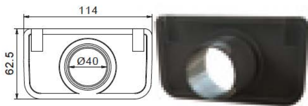
END-CAP 100/55
