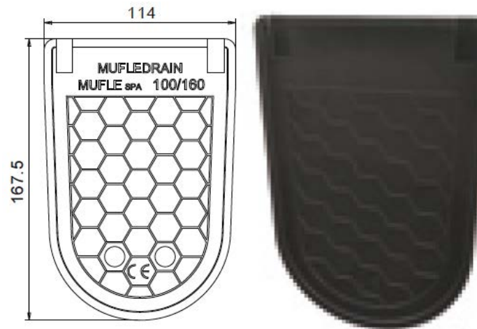
CLOSED END-CAP WITH DRAIN 100/160
