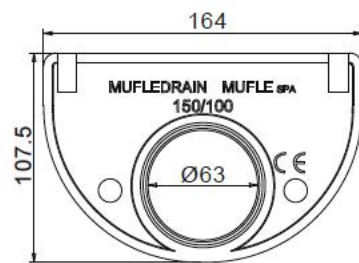
END-CAP 150/100
