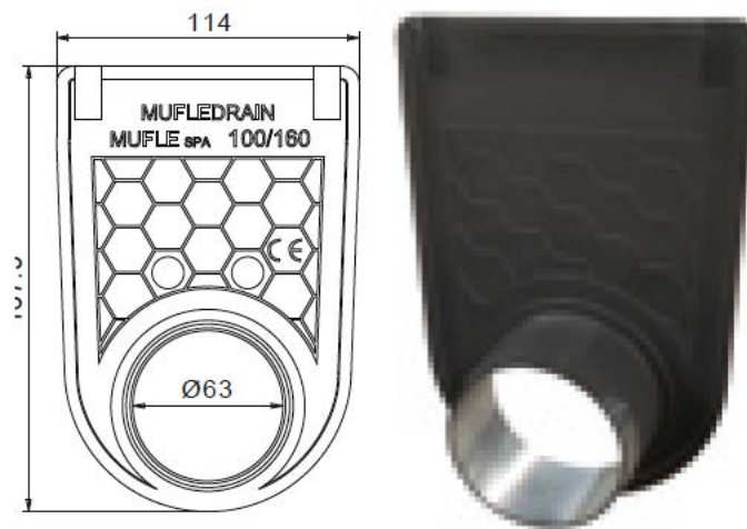
END-CAP 100/160
